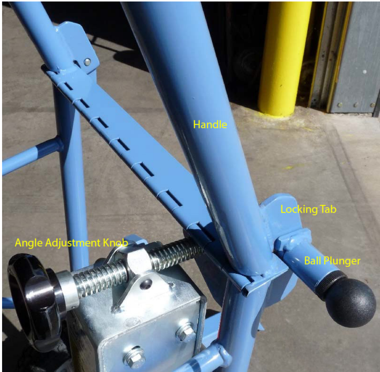
Figure 2 above shows a Back Buddy II™.
