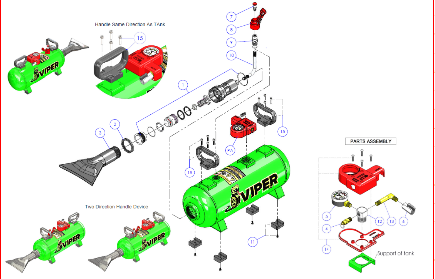
VP-18AL GEN 3.0 Main Assembly
